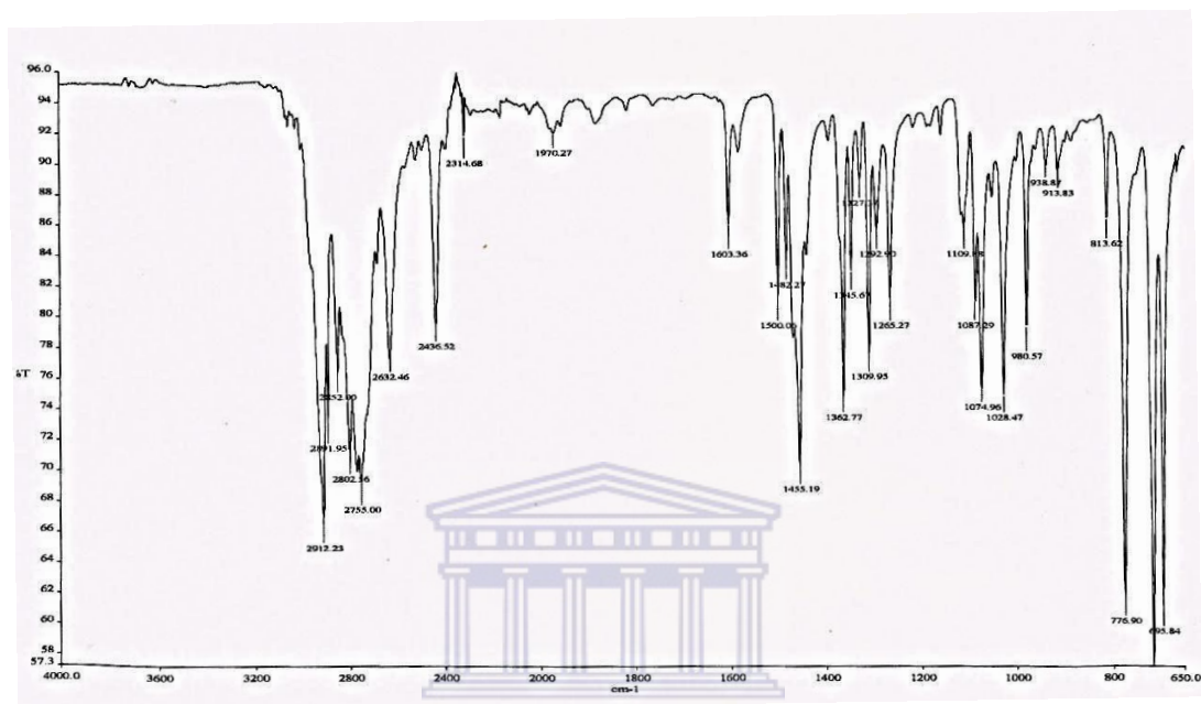
Spectrum 32: IR spectrum of SE-11
