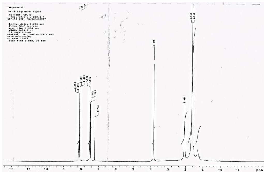
Spectrum 13: 1 H NMR spectrum of SE-4
