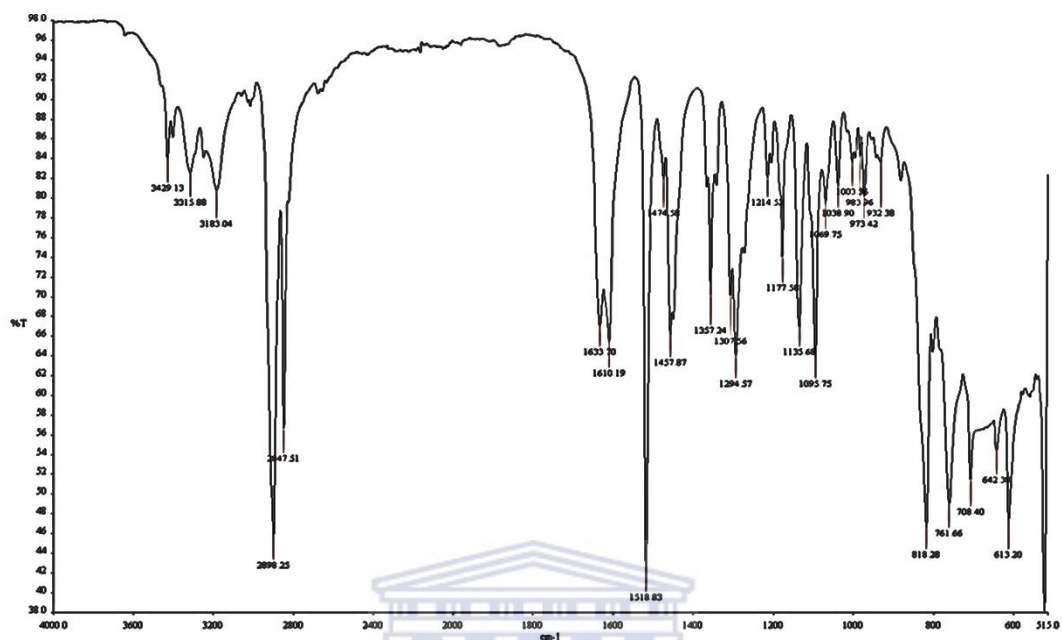
Spectrum 28: IR spectrum of SE-7
