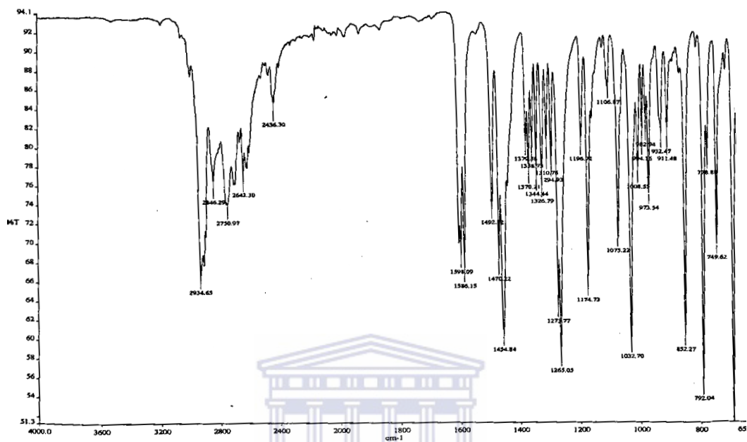
Spectrum 40: IR spectrum of SE-13
