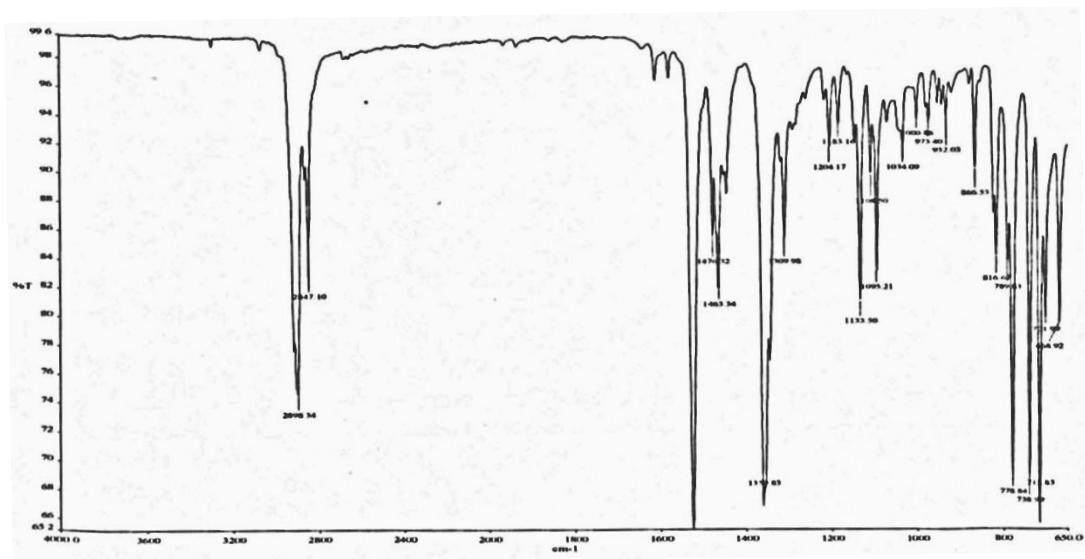
Spectrum 12: IR spectrum of SE-3
