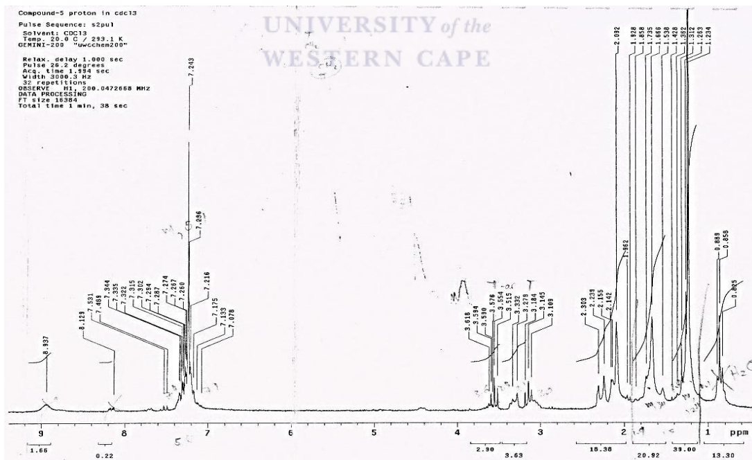
Spectrum 29: 1 H NMR spectrum of SE-11
