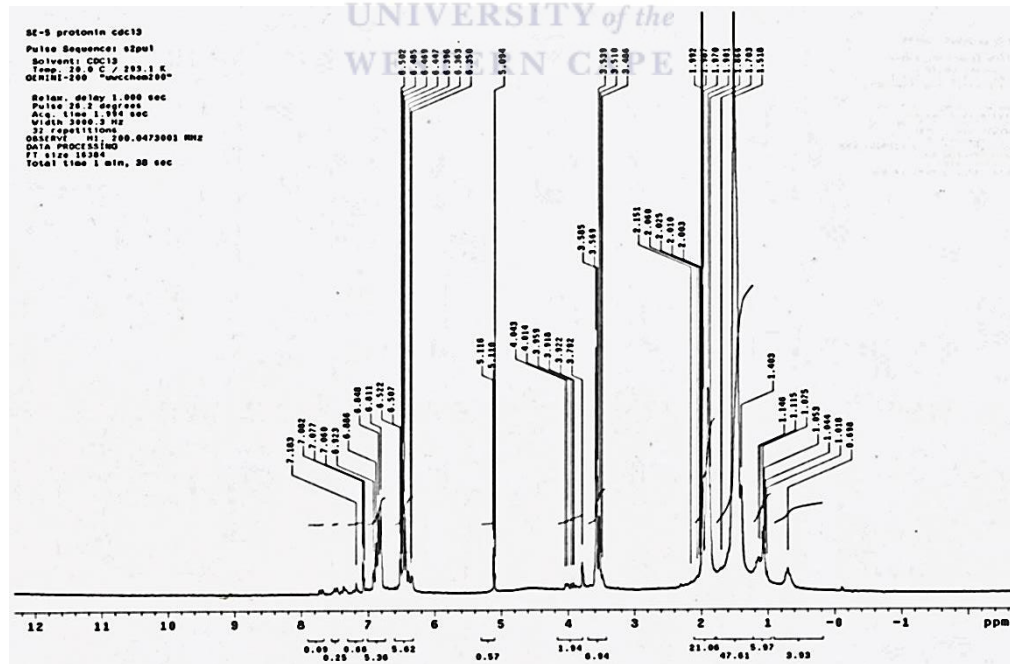
Spectrum 17: 1 H NMR spectrum of SE-5
