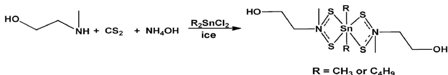
Figure 1. Synthetic scheme of the alkyltin(IV) N -methyl- N -hydroxyethyl dithiocarbamate complexes.
